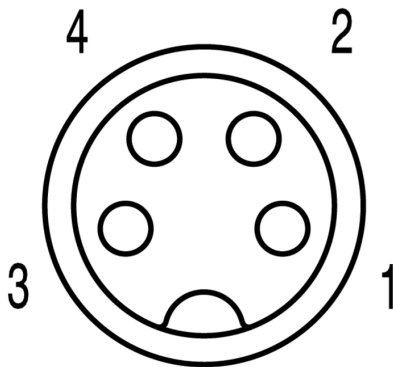
Female contact
