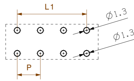
HOLE PATTERN
